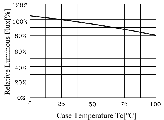
Case Temperature Vs. Relative Luminous Flux
